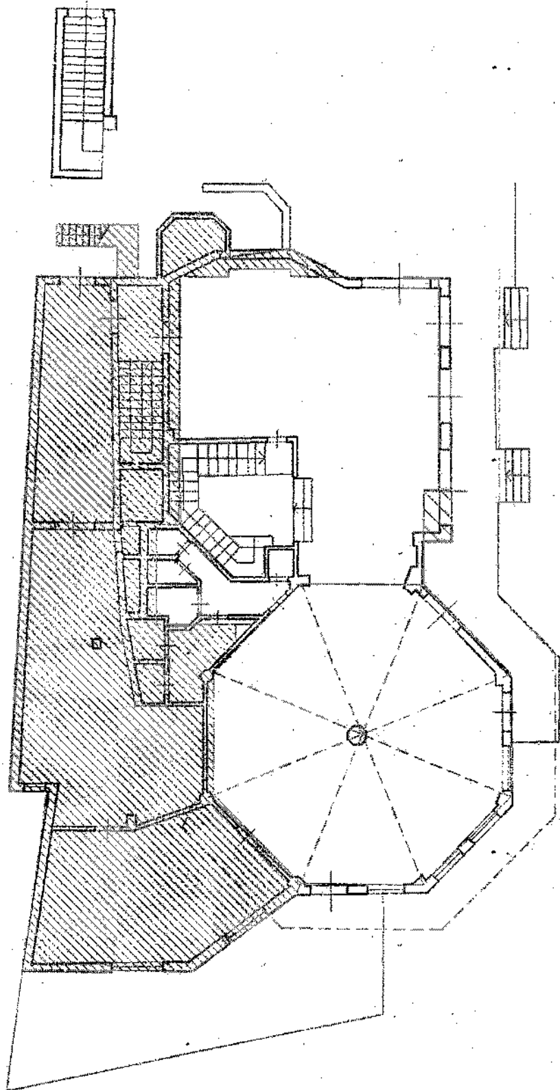
PIANO TERRA H=3,05 m 2
